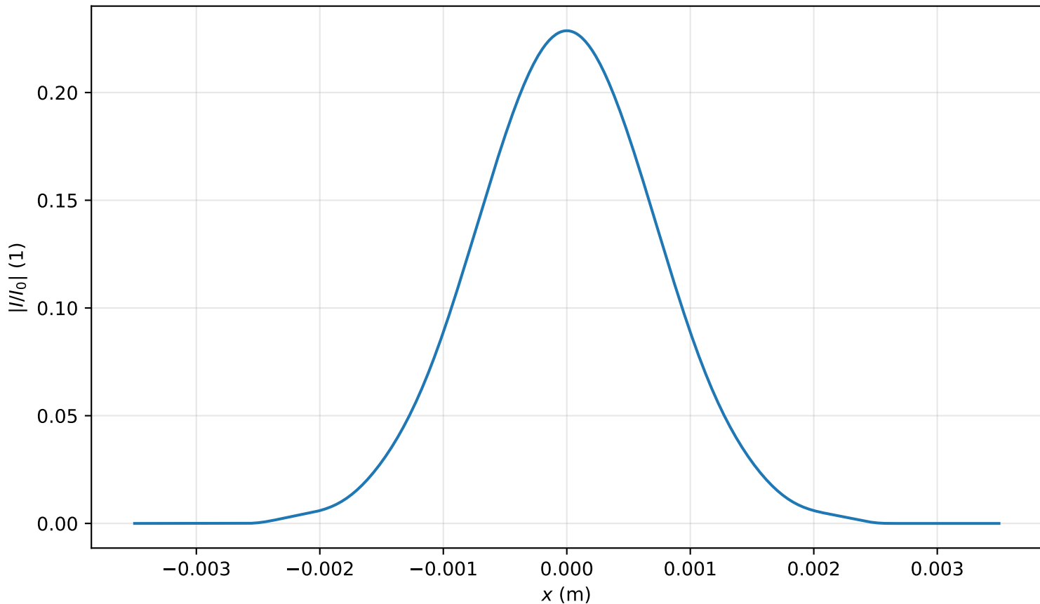
Intensity profile I(x, y = 0, z = 3.901m)/I_0 , P_{in}=0.1P_{cr} , artificial time
